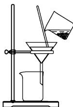
C. 分离 \text{NaHCO}_3
